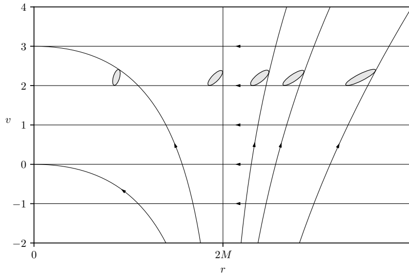
Figure 8.1: Photon world lines in (v, r) spacetime diagram. Several future light cones are drawn. The arrows indicates the direction of world lines in increasing t : the horizontal lines represent v = t + r^* = \text{const.} , where increasing t means decreasing r^* or r ; the curved lines represent the outgoing null geodesics u = v - 2r^* = \text{const.} . Increasing t means increasing r^* , or increasing r for r > 2M , and decreasing r for r < 2M (so the “outgoing” photon is traveling inward towards r = 0 inside r = 2M ).
