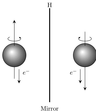
Figure 5.1: Decay of Cobalt 60 (left) and its mirror image (right). In the beta decay of Cobalt 60, most electrons are emitted in the direction opposite to the nuclear spin.
