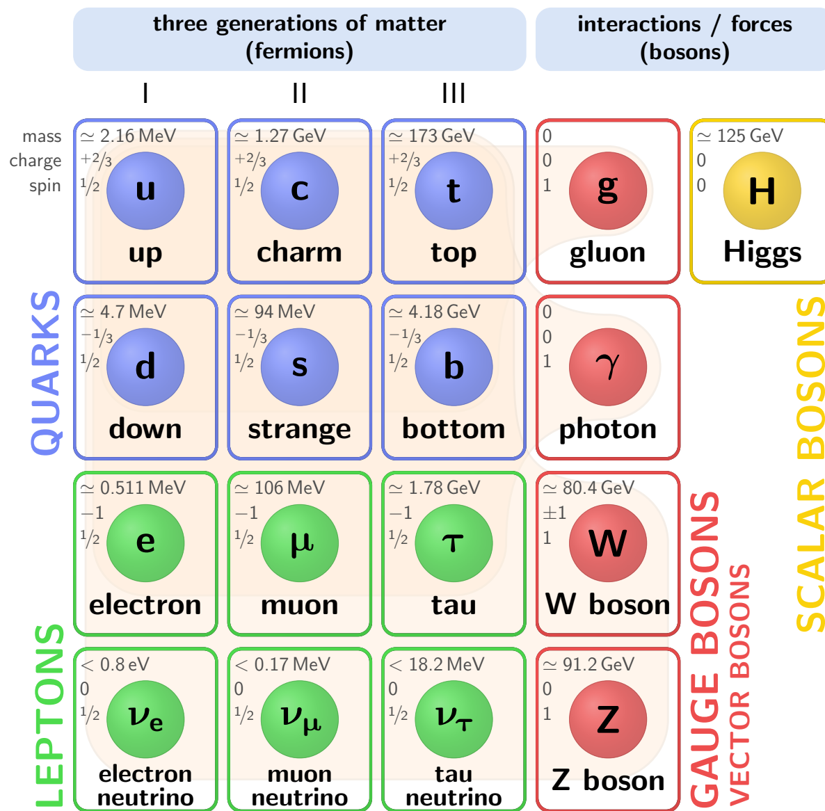
Figure 1.1: The table of the Standard Model. This is definitely not the best figure for particle categorization in the Standard Model. It is misleading that these elementary particles are drawn as spheres while they are commonly known to be pointlike. Also, particles in the same row somehow suggests that they have something in common. This is not the case, as u , c , and t are not more connected to the gluon and Higgs boson than d , s , and b are.
