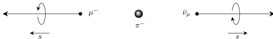
Figure 5.2: Decay of \pi^- at rest.
