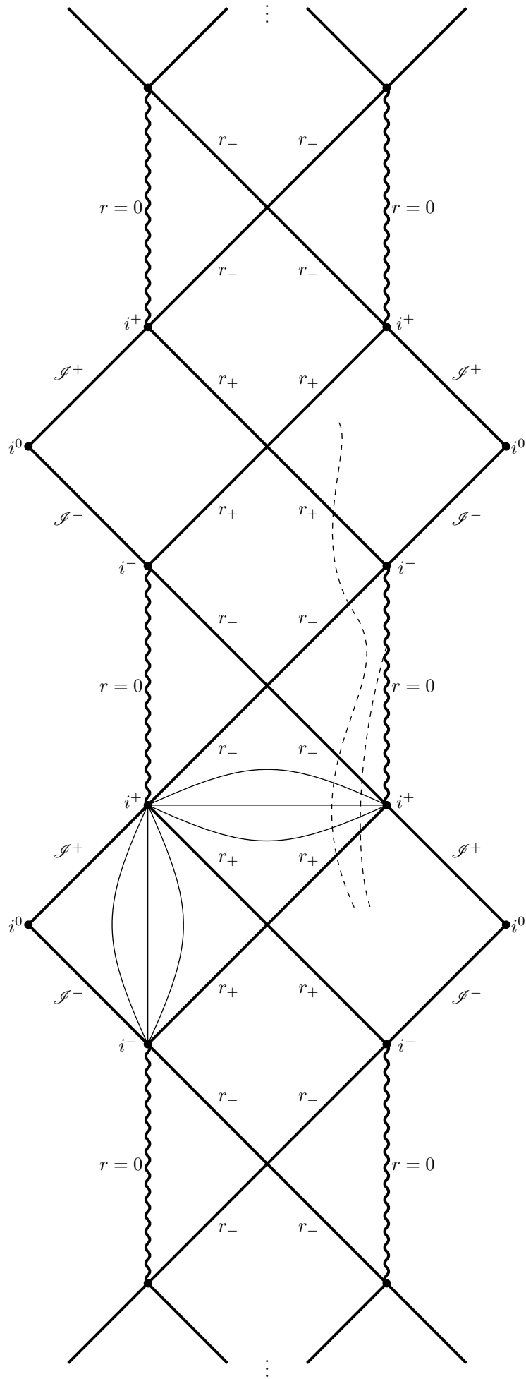
Figure 8.6: Penrose diagram of the Reissner-Nordström solution with Q^2 < M^2 . r = \text{const.} surfaces are shown in thin solid lines. Two possible timelike trajectories are shown in dashed lines.
