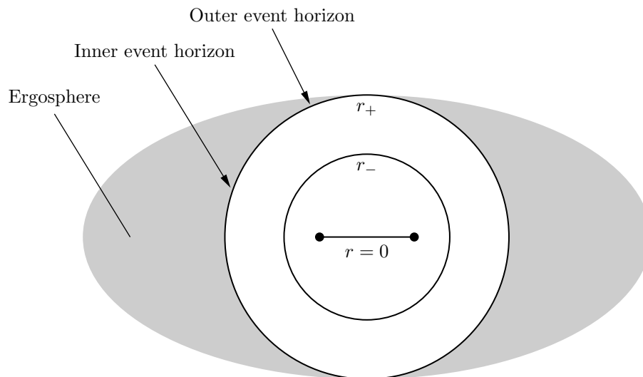
Figure 8.8: The structure of a Kerr black hole (side view) with M > a . There are two event horizons located at r = r_{\pm} . The curvature singularity r = 0 and \theta = \pi/2 is a ring. Outside the outer horizon is the ergosphere where no observer can remain stationary.
