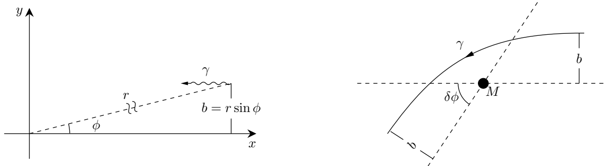
Figure 7.4: Interpretation of b as the impact parameter for a photon from infinity (left) and gravitational light bending (right).
