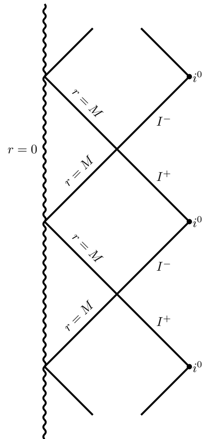
Figure 8.7: Penrose diagram of the extreme Reissner-Nordström solution.
