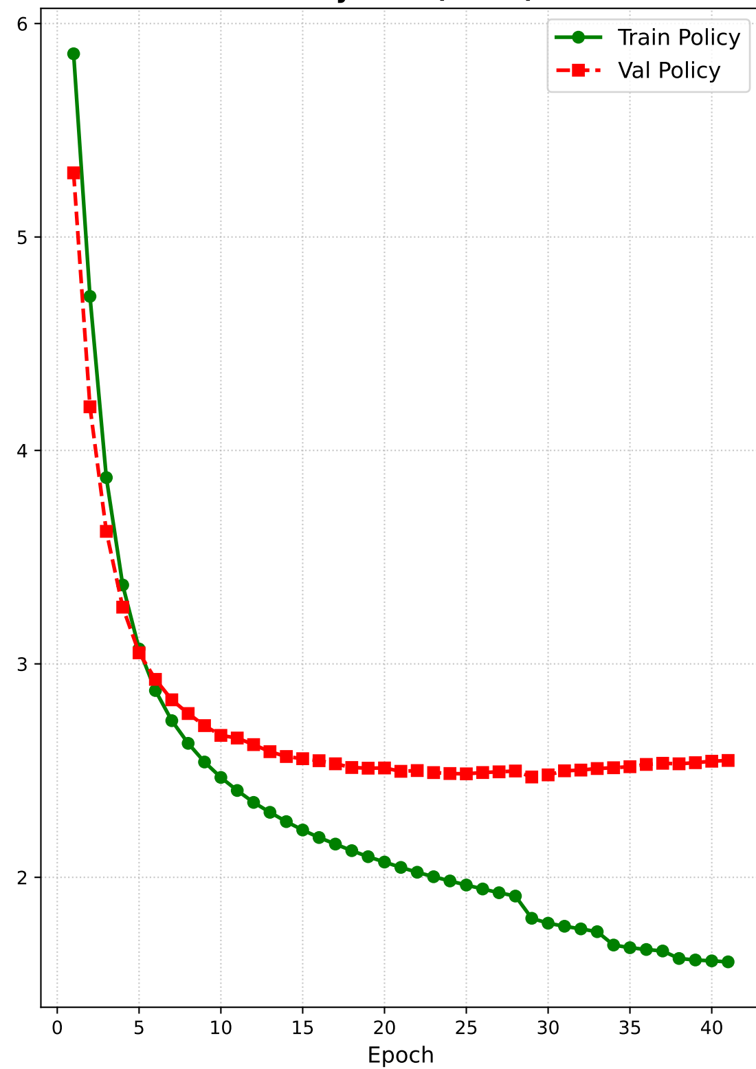
Policy Loss (Actor)
