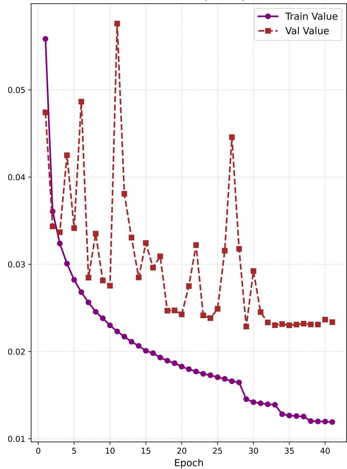
Value Loss (Critic)
