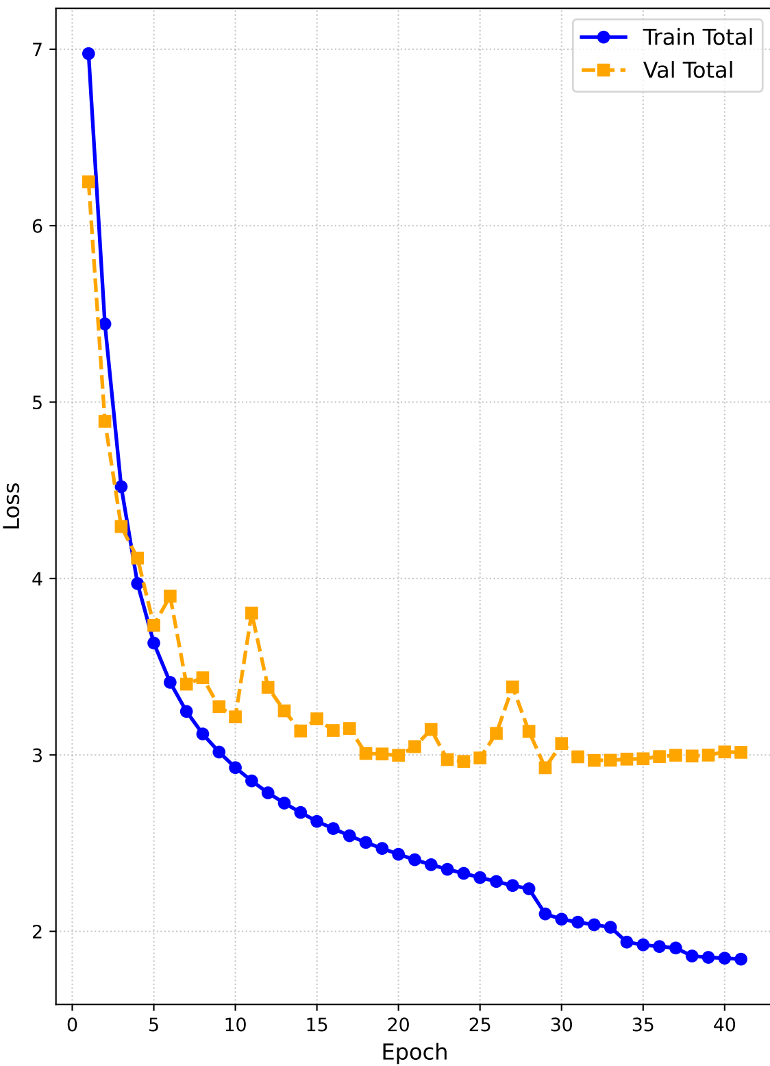
Total Combined Loss
