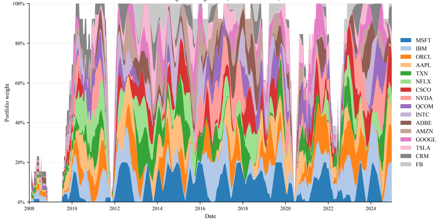
Portfolio Weights Through Time (13-week smoothed)
