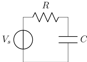
Figure 10.3: Simple RC circuit drawn with circuitikz .
