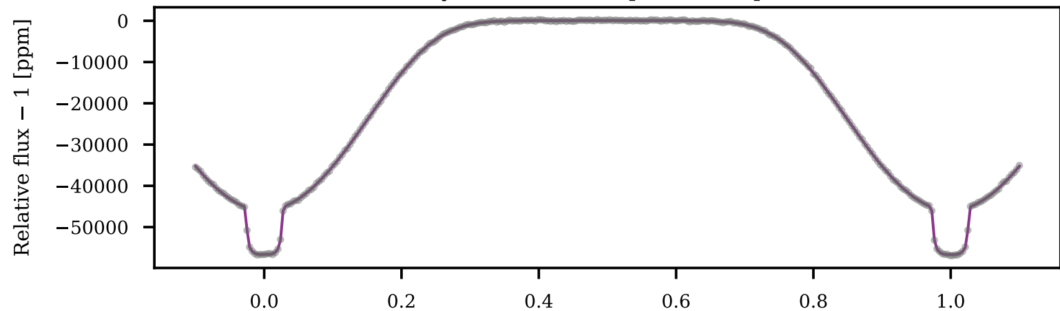
Synthetic stellar spots · 4.03 \mu\text{m}
