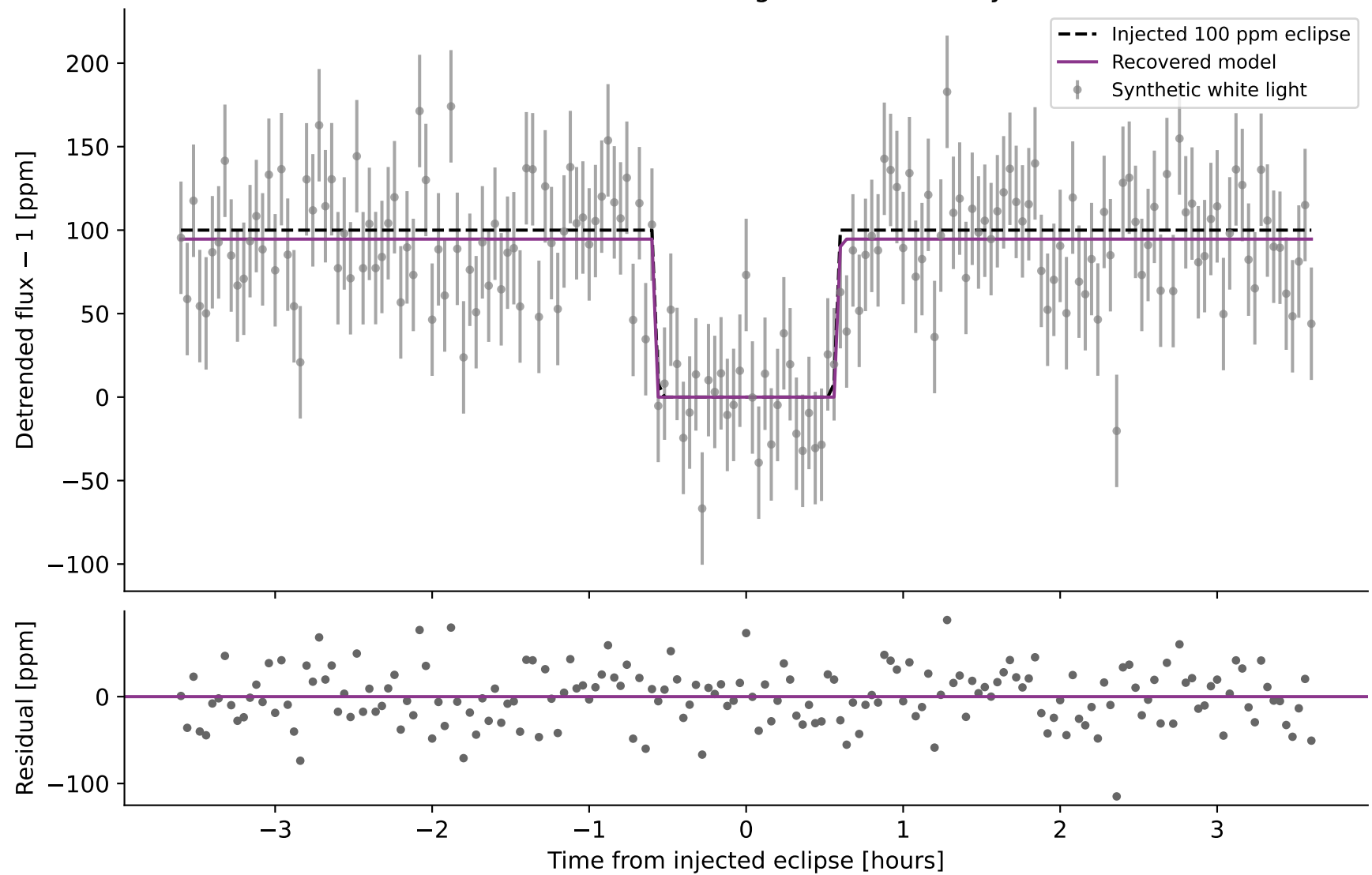
ROCKY-1 b · native-grid GPU recovery
