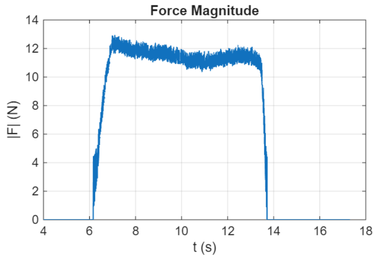
Fig. 8. Single-depth virtual wall contact test. The rendered |F| remains steady during sustained contact, with mean 11.46 N, standard deviation 0.30 N, and coefficient of variation 0.026.
