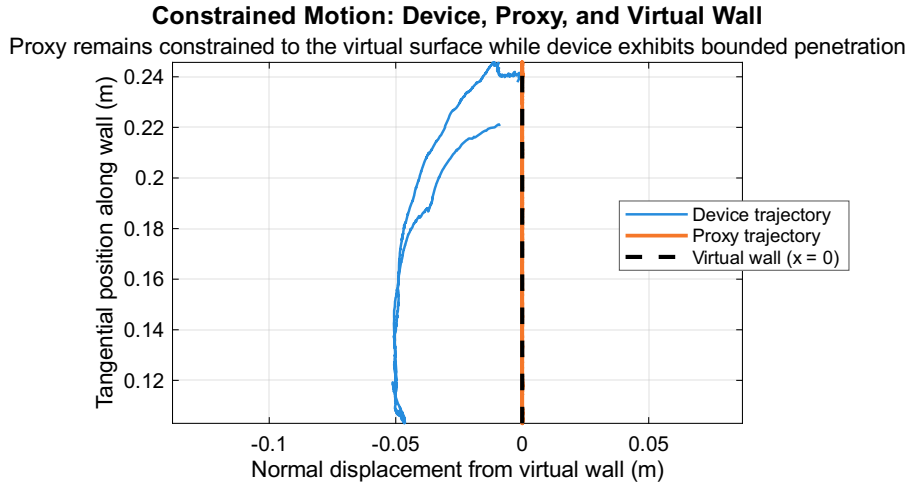
Fig. 15. Device and proxy trajectories during the analysed constrained-motion window from 20.50 s to 23.20 s. The proxy remains constrained to the wall while device normal displacement stays bounded.
