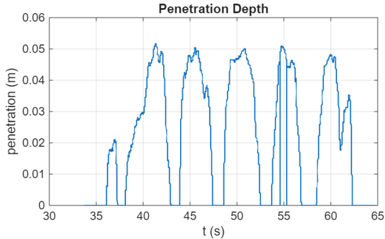
Fig. 14. Motor-enabled repeated contact test. Maximum penetration was approximately 0.052 m; the force–penetration fit gave 490.99 \text{ N m}^{-1} with R^2 = 0.9979 .
