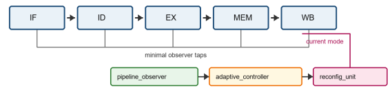
PipeSense-ARM closed-loop pipeline
