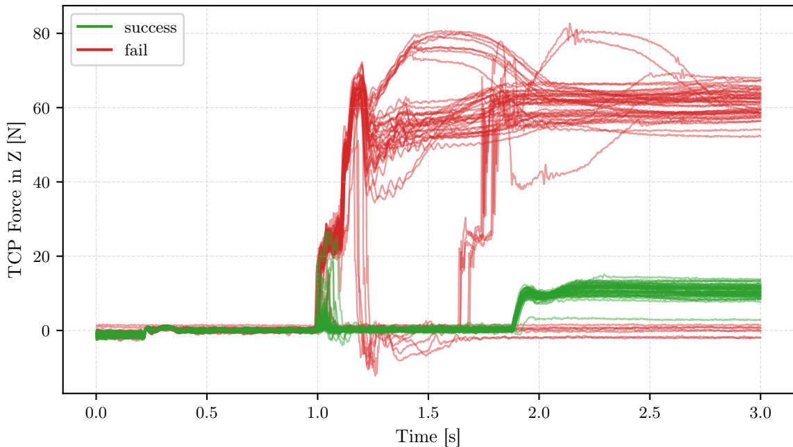
TCP Force in Z of batch_1/big_rod_t0.1 over 100 insertions with a split of Success: 51, Fail: 49
