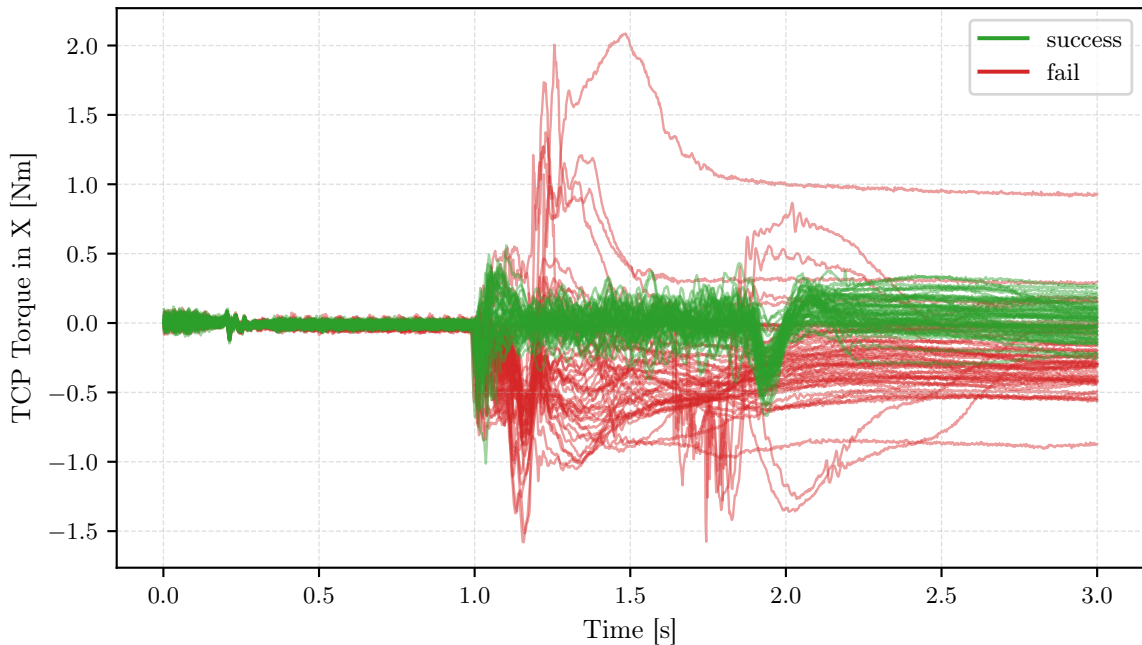
TCP Torque in X of batch_1/big_rod_t0.1 over 100 insertions with a split of Success: 51, Fail: 49
