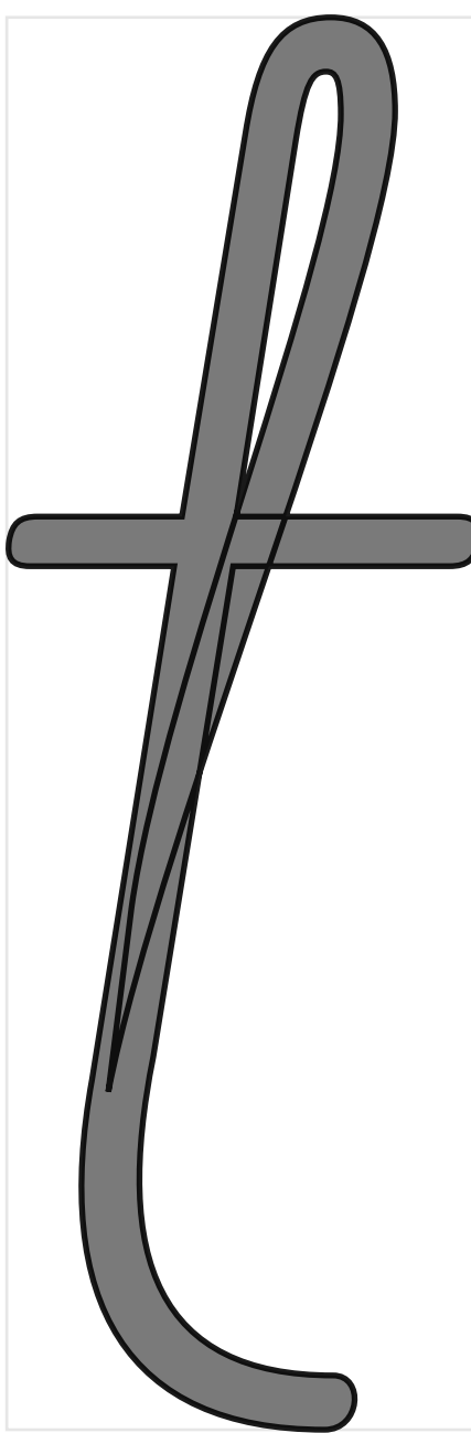
midway interpolation
