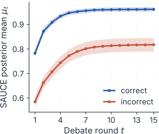
SAUCE: gap persists
