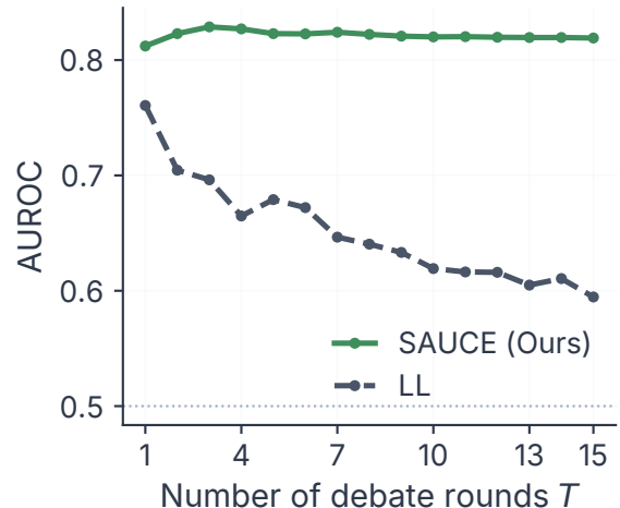
AUROC vs debate length
