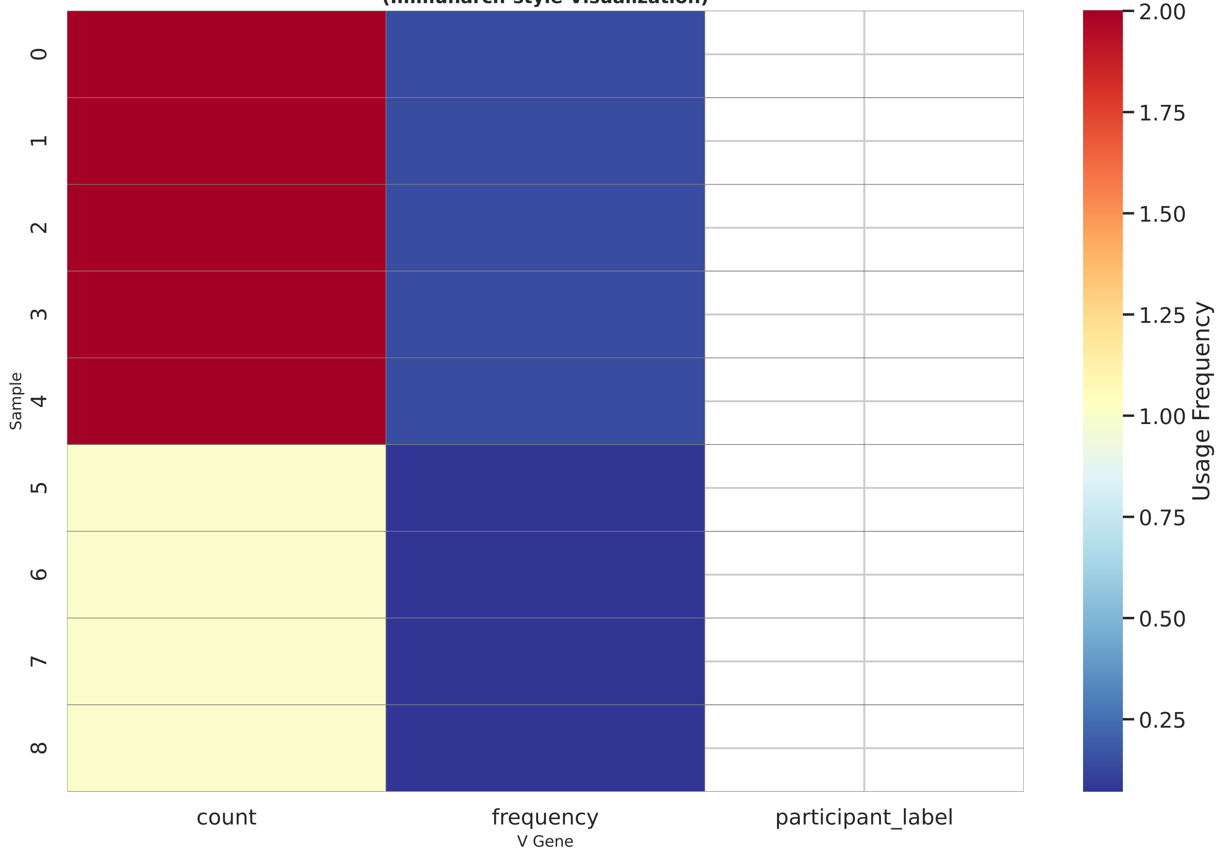
V Gene Usage Heatmap (Immunarch-style Visualization)
