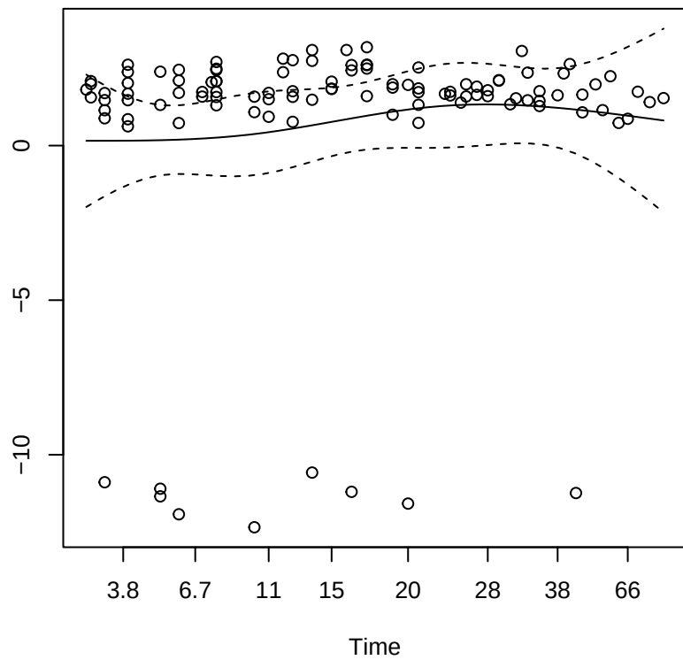
Beta(t) for mmr
