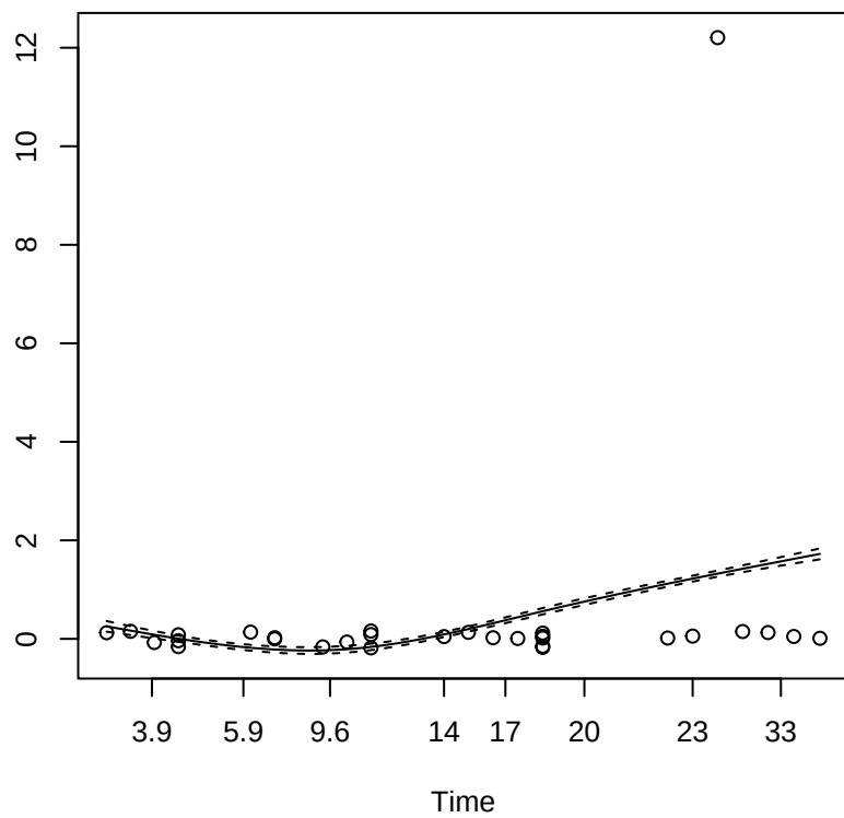
Beta(t) for age
