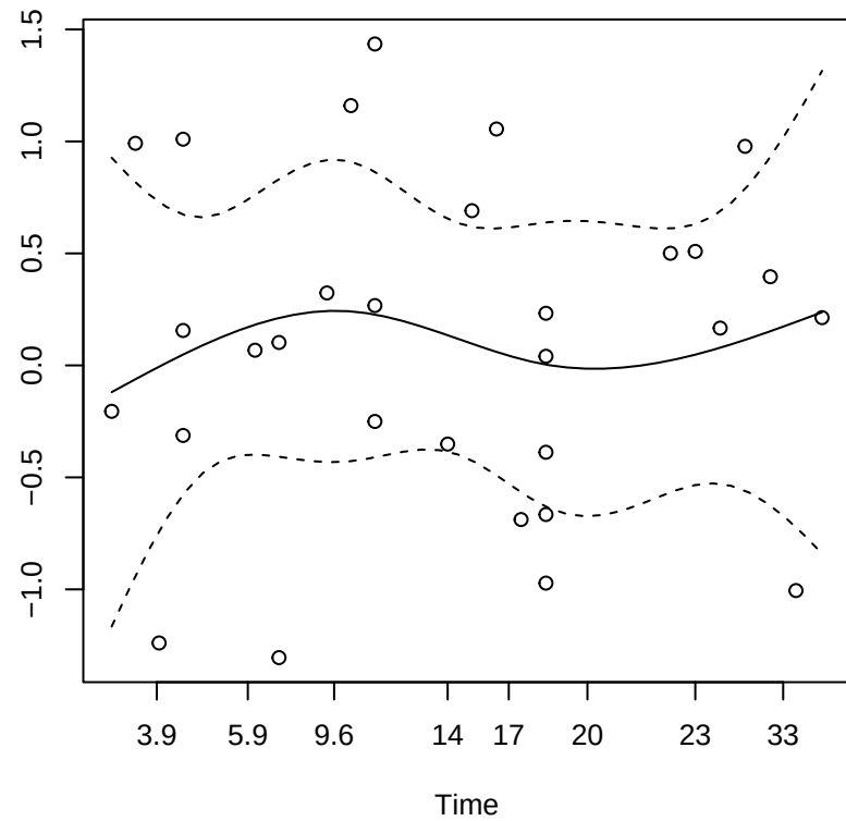
Beta(t) for score_z
