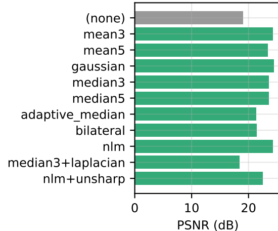
gaussian_s30
