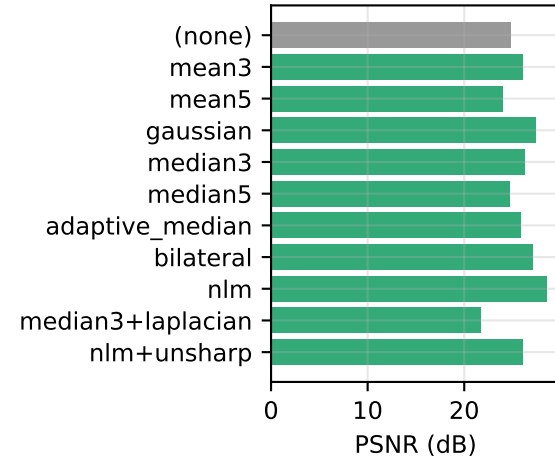
gaussian_s15
