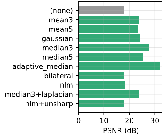
saltpepper_5
