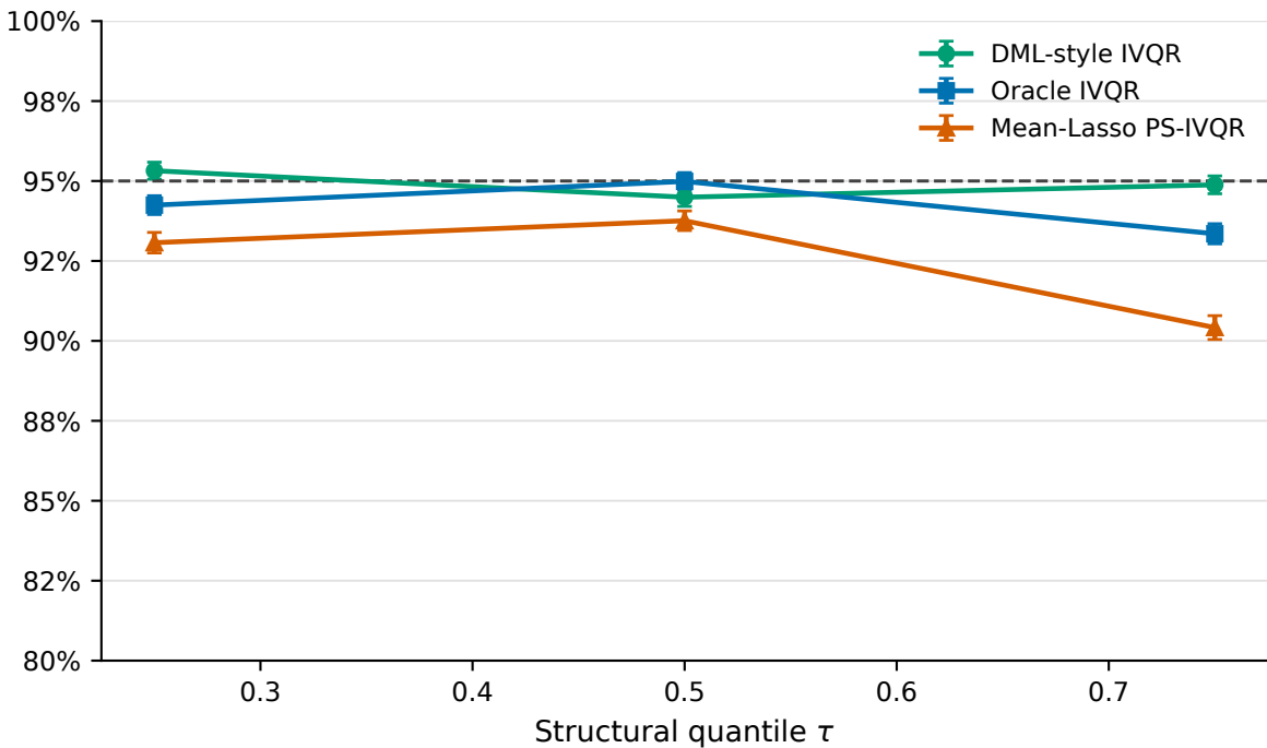
Resolved-replication coverage
