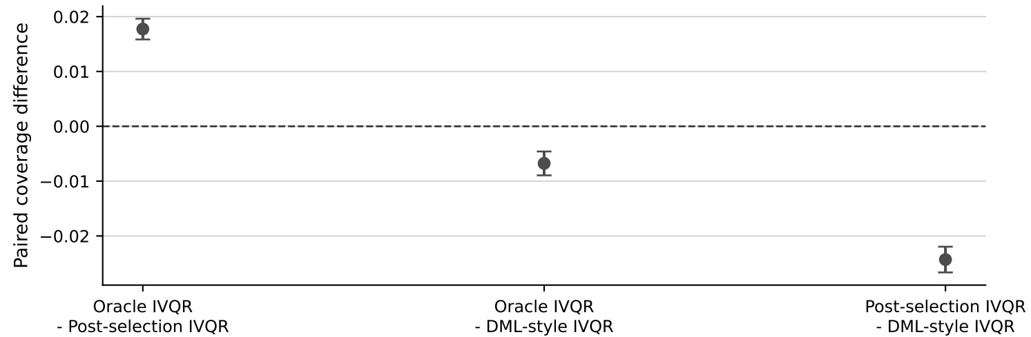
Difference orientation: estimator A - estimator B
