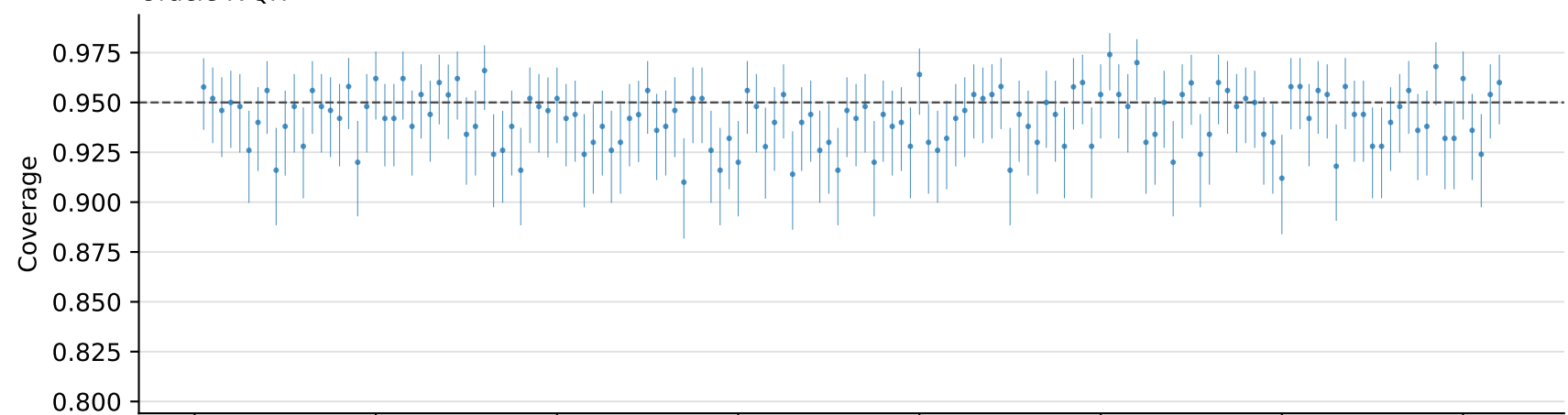
Post-selection IVQR
