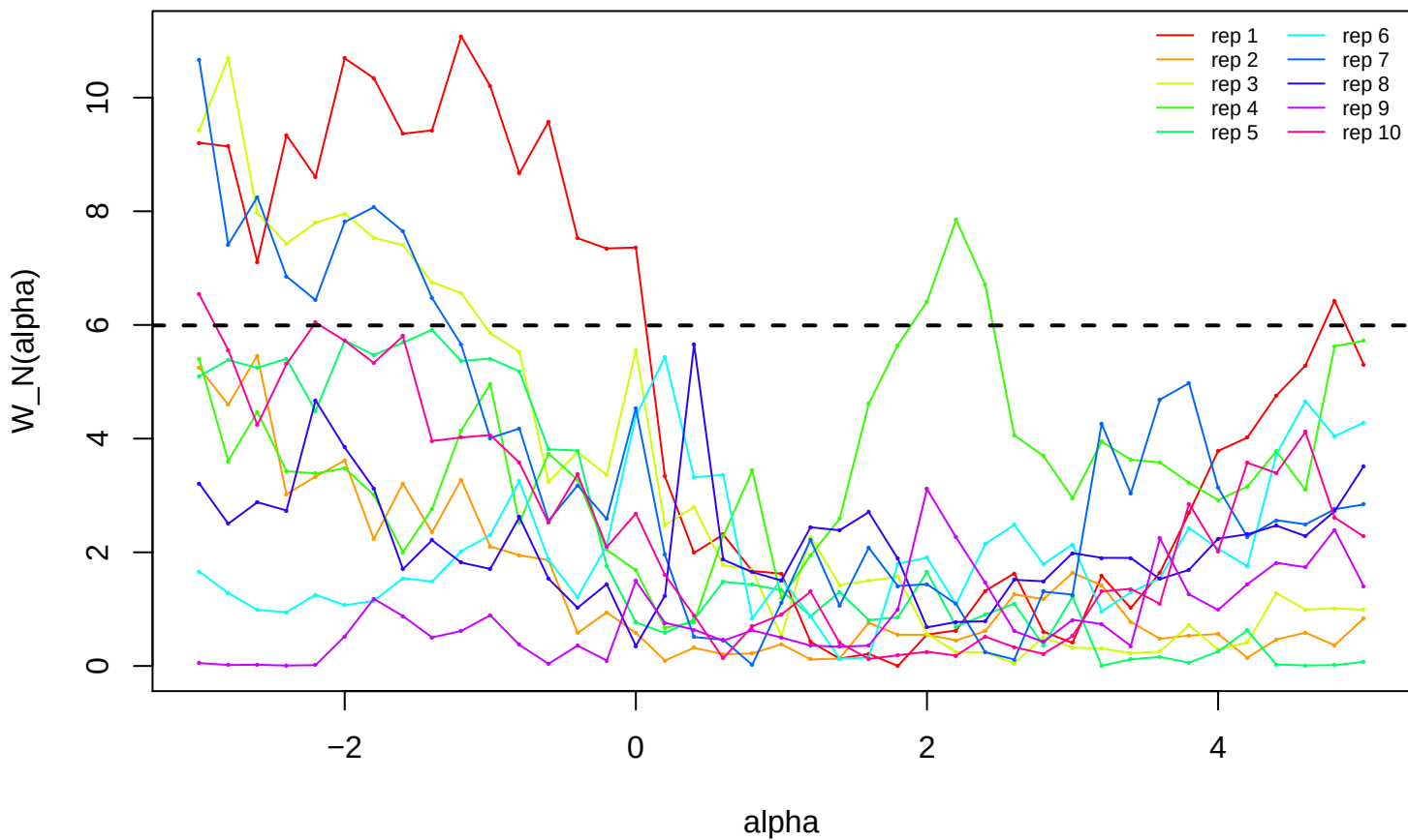
DML-IVQR tau = 0.50 kappa = 0.10, n = 500
