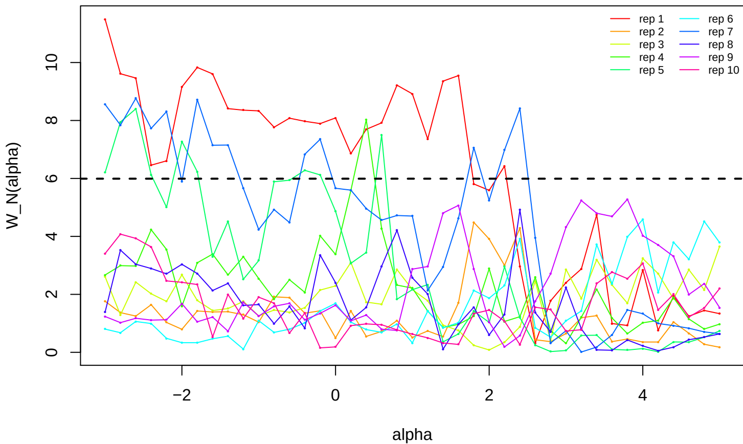
DML-IVQR tau = 0.90 kappa = 0.10, n = 500
