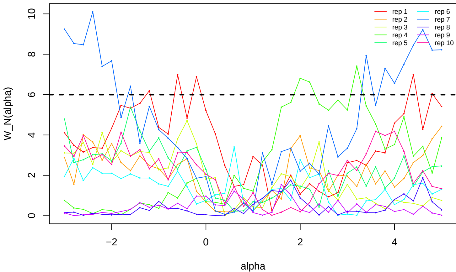
Oracle-GMM tau = 0.50 kappa = 0.10, n = 500
