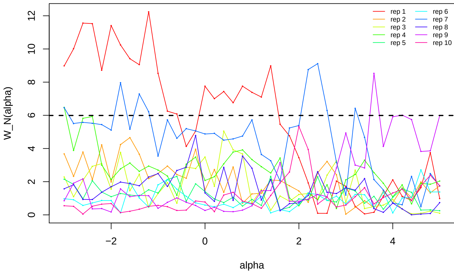
Oracle-GMM tau = 0.90 kappa = 0.10, n = 500
