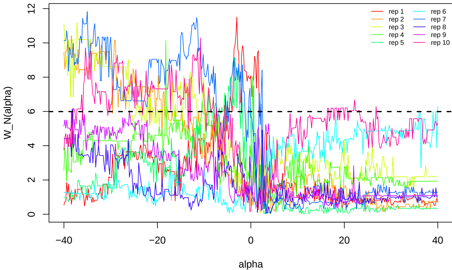
DML-IVQR tau = 0.90 [-40,40]
