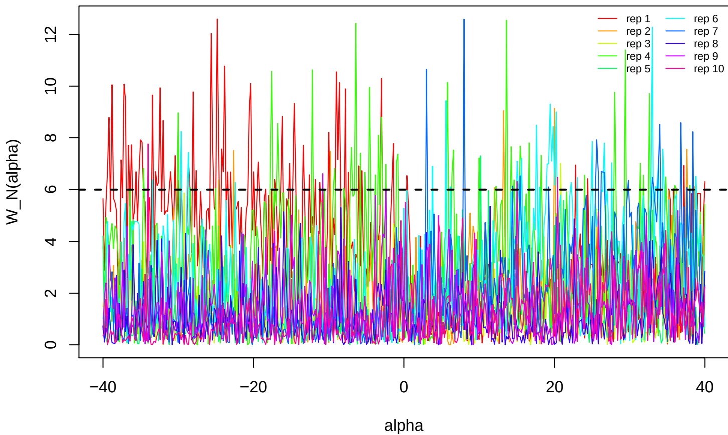
Full-GMM tau = 0.10 [-40,40]
