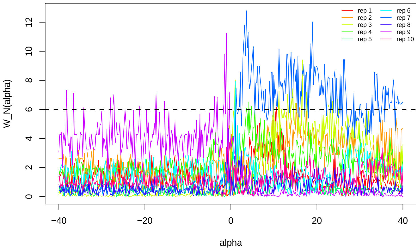
Oracle-GMM tau = 0.10 [-40,40]
