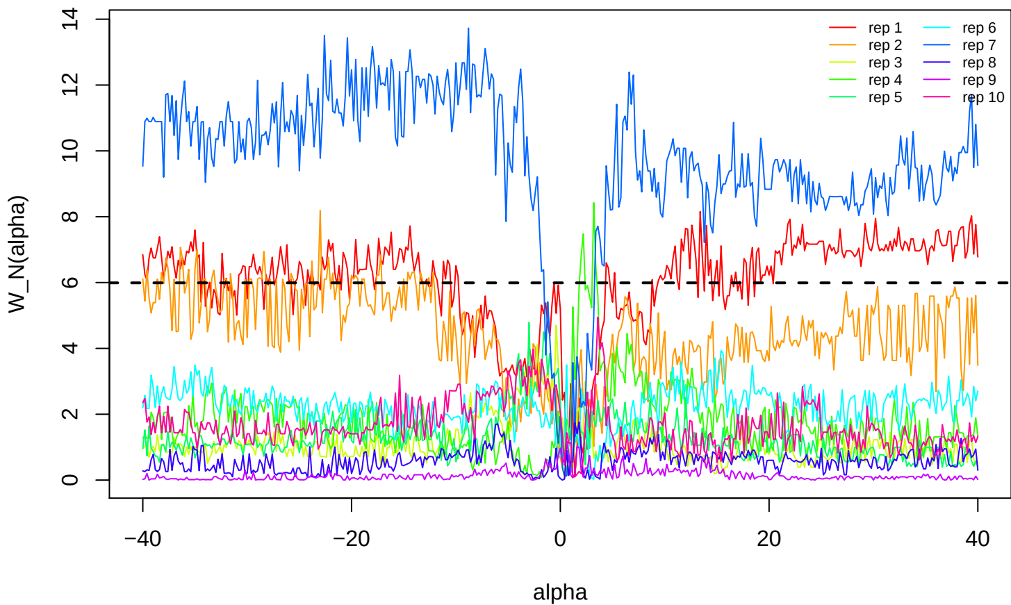
Oracle-GMM tau = 0.50 [-40,40]
