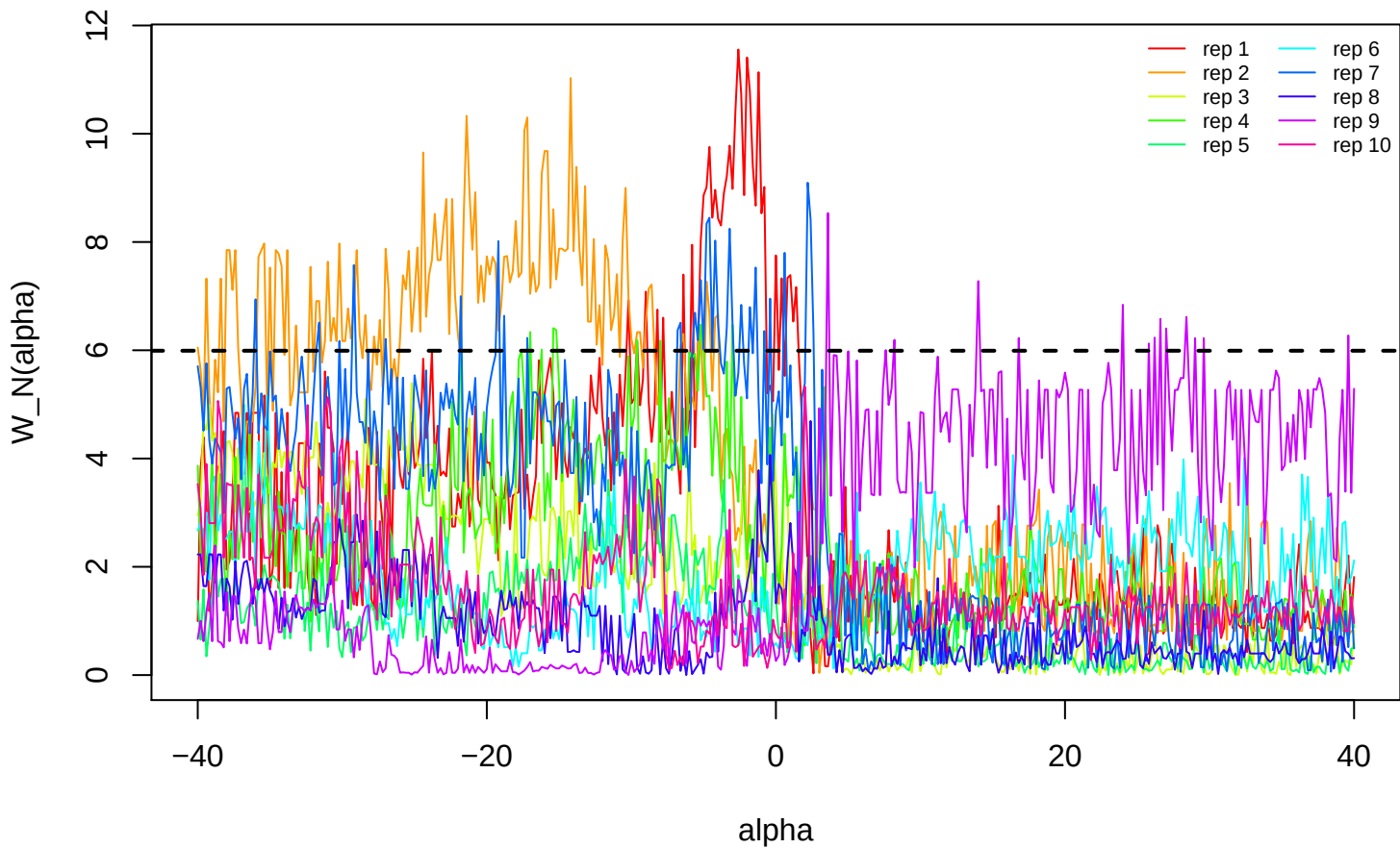
Oracle-GMM tau = 0.90 [-40,40]
