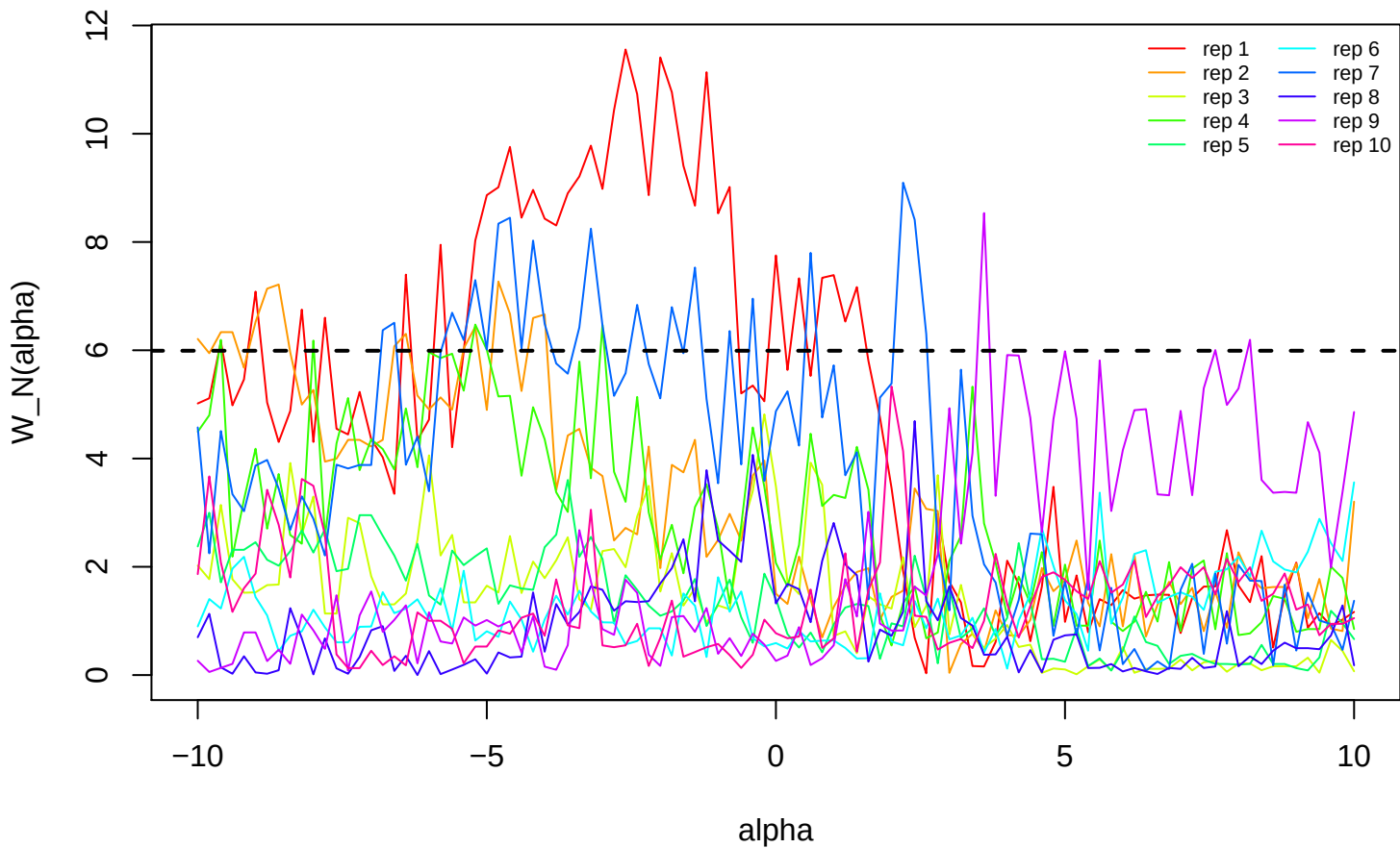
Oracle-GMM tau = 0.90 [-10,10]
