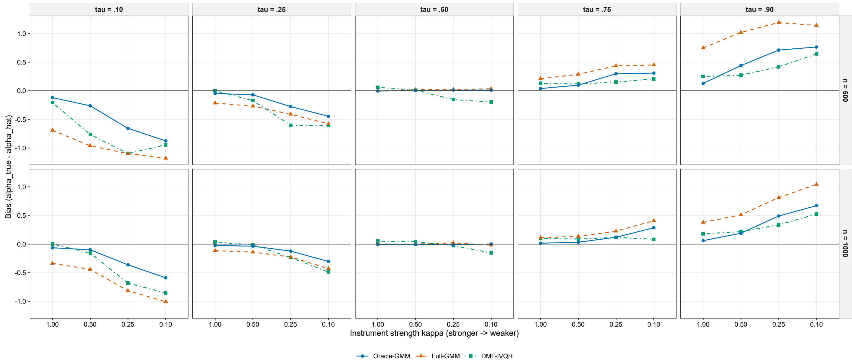
Bias across instrument-strength designs
