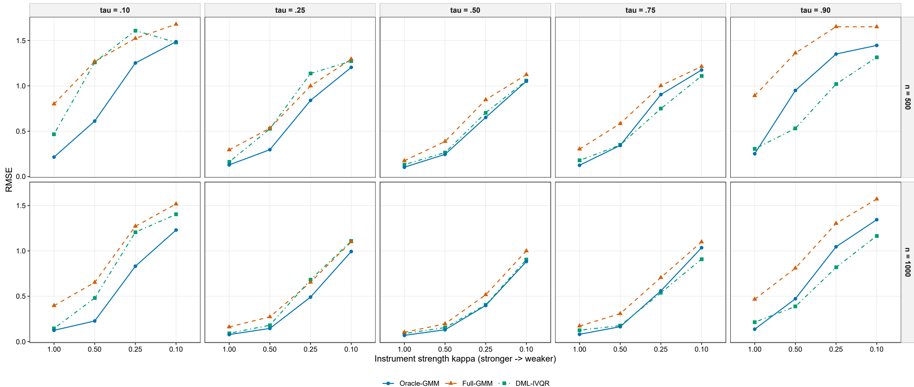
RMSE across instrument-strength designs
