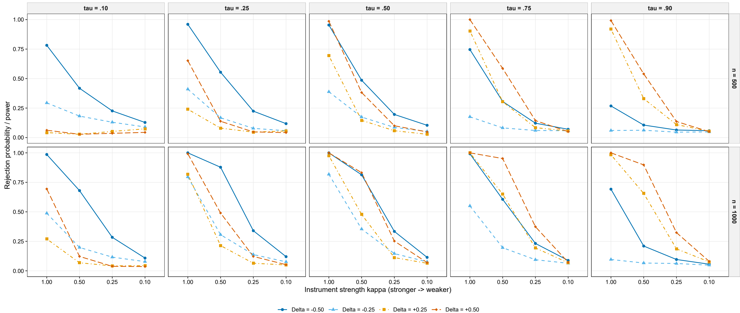
DML-IVQR power across directional alternatives
