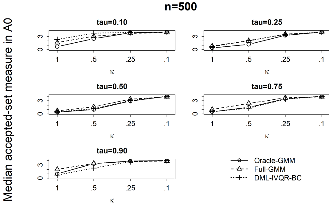
Figure 2. Grid-based accepted-set measure within the primary computational domain A_0 = [-1, 3] , n = 500
