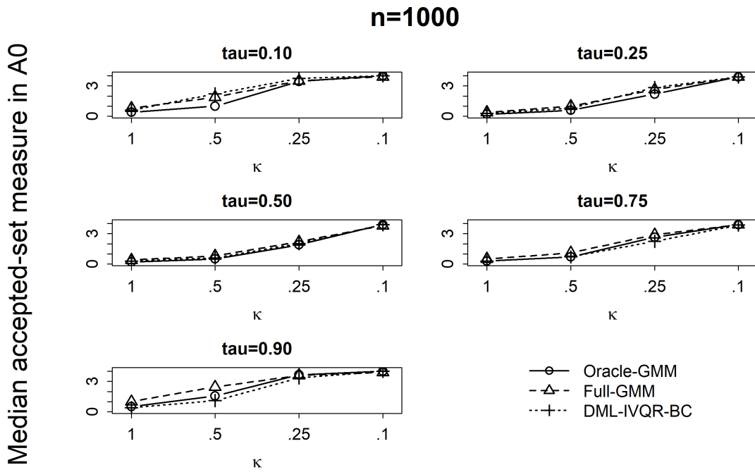
Figure 3. Grid-based accepted-set measure within the primary computational domain A_0 = [-1, 3] , n = 1000
