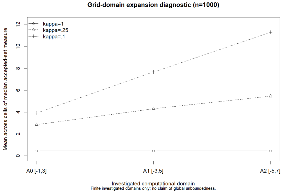
Figure 1. Sensitivity of the accepted set to expansion of the computational domain
