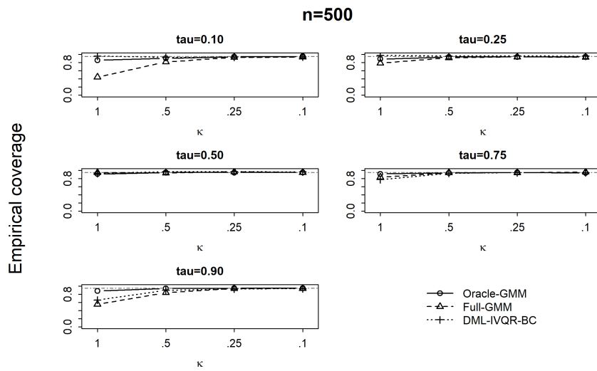
Figure 5. Empirical coverage across instrument-strength designs, n = 500
