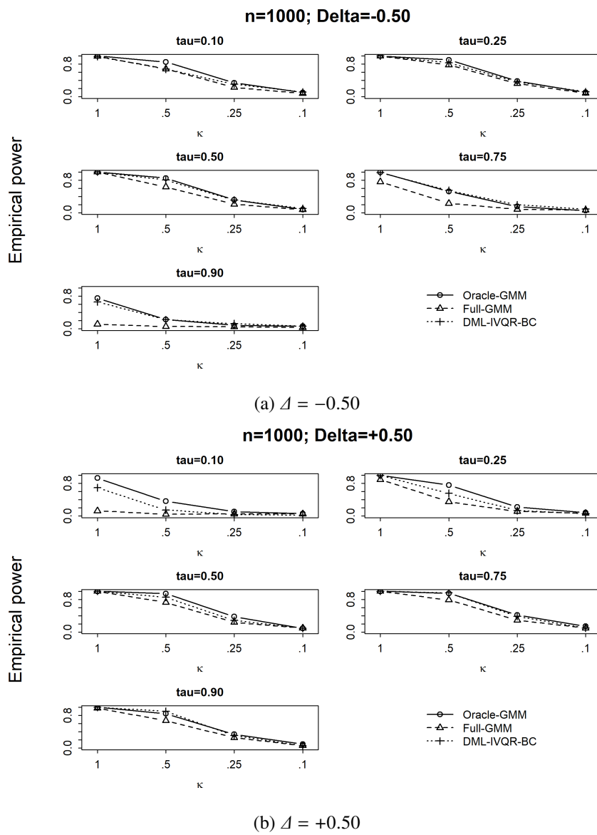
Figure 4. Rejection probability under moderate false alternatives, n = 1000
