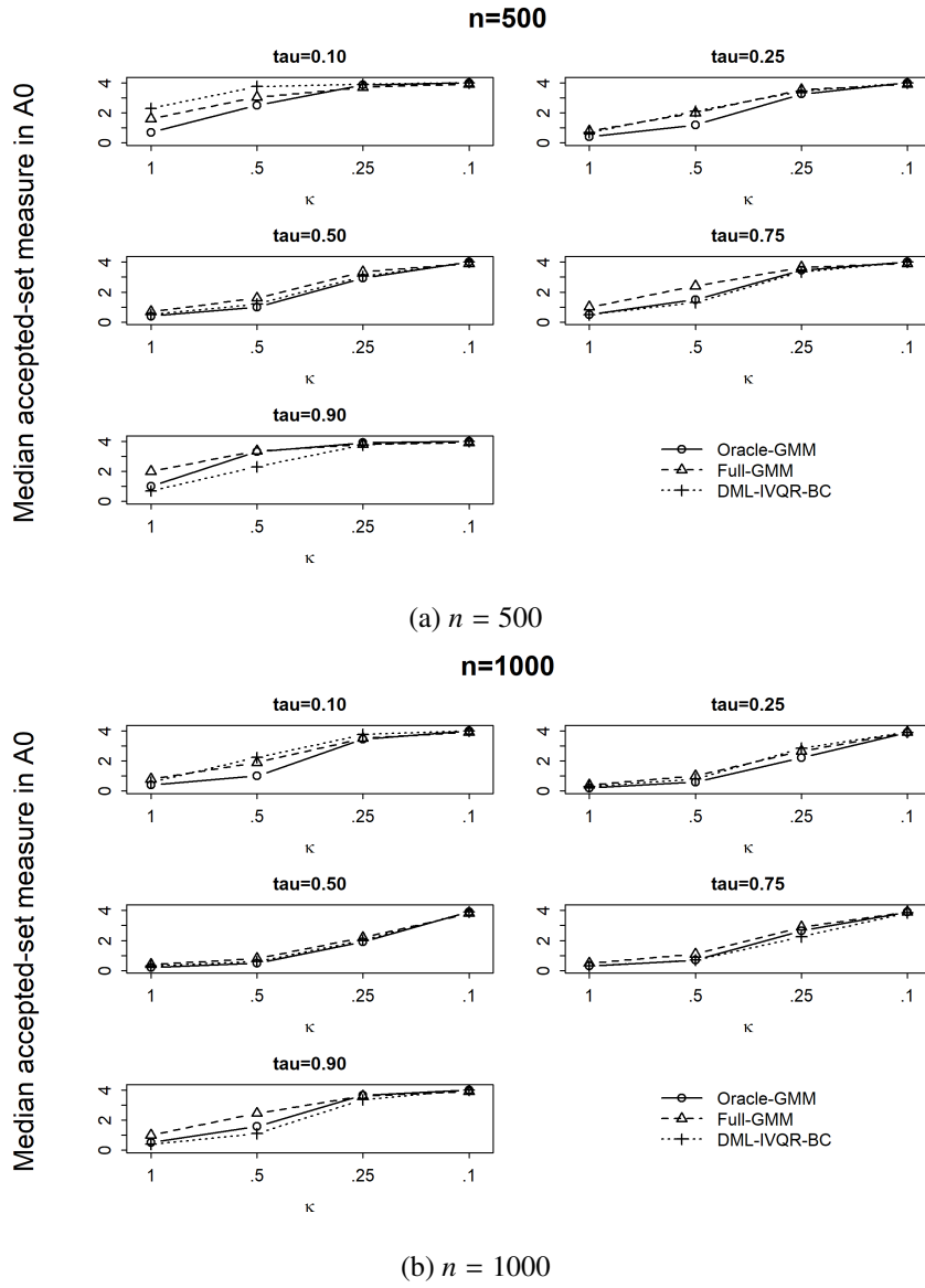
Figure 3. Grid-based accepted-set measure within the primary computational domain A_0 = [-1, 3]
