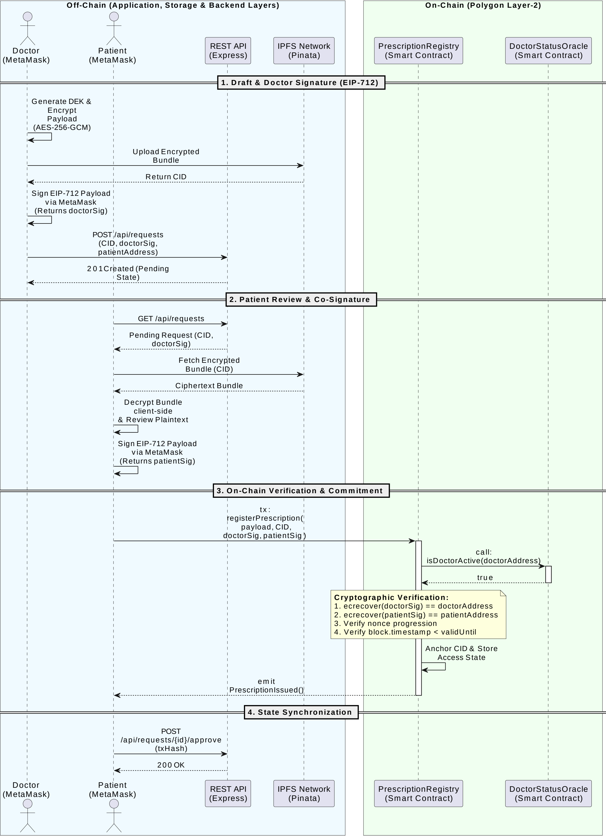
Figure 4.1: Granular Dual-Signature (EIP-712) Workflow
