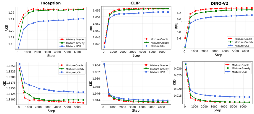
Figure 3: Convergence of RKE and KD on FFHQ generative models, using different feature extractors.
