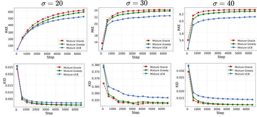
Figure 2: Convergence of KD and RKE for generative models trained on FFHQ dataset using three bandwidths
