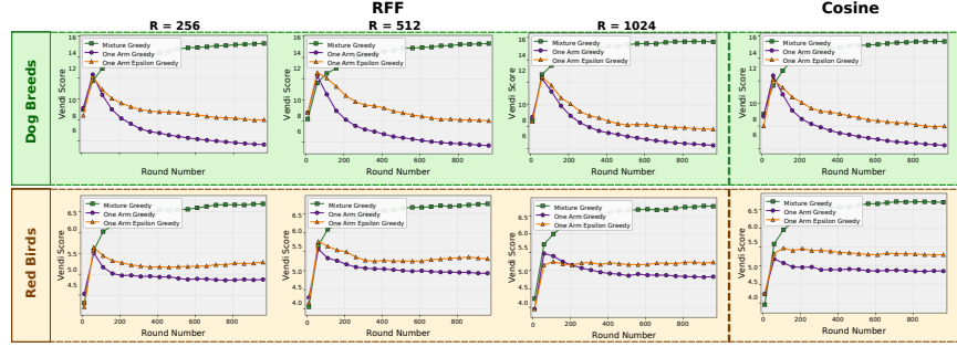
Figure 1: Vendi score over rounds for different using RFF (R=256/512/1024) and cosine kernel on two generated datasets.
