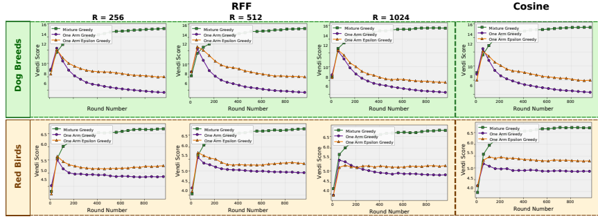
Figure 2: Vendi score over rounds for different using RFF (R=256/512/1024) and cosine kernel on two generated datasets.
