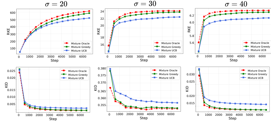
Figure 3: Convergence of KD and RKE for generative models trained on FFHQ dataset using three bandwidths
