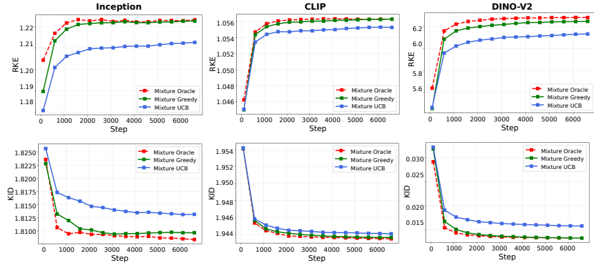
Figure 4: Convergence of RKE and KD on FFHQ generative models, using different feature extractors.
