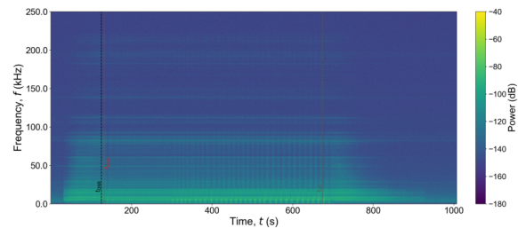
(b) P_{\text{load}} = 250 \text{ W}
