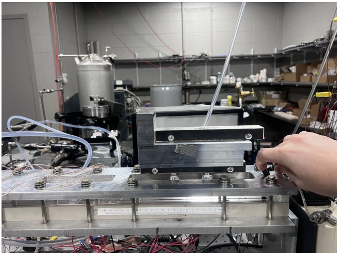
(c) Heated test section and surface sensors
