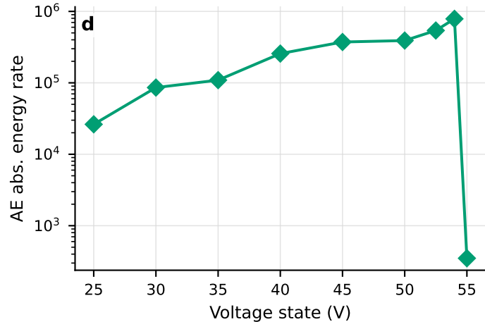
AE activity, provisional alignment
