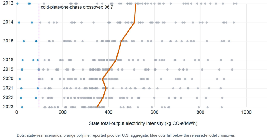
Figure 3: Harmonized AR5-GWP100 eGRID state/DC generation rates for nine releases, with electricity intensity on the horizontal axis in kg CO 2 e/MWh. The orange poly-line connects the reported provider U.S. aggregate for each year. Blue points fall below the released-workbook numerical cold-plate/single-phase crossover. These are direct-generation scenarios, not consumption LCIs, state cooling LCAs, or facility decision thresholds.
