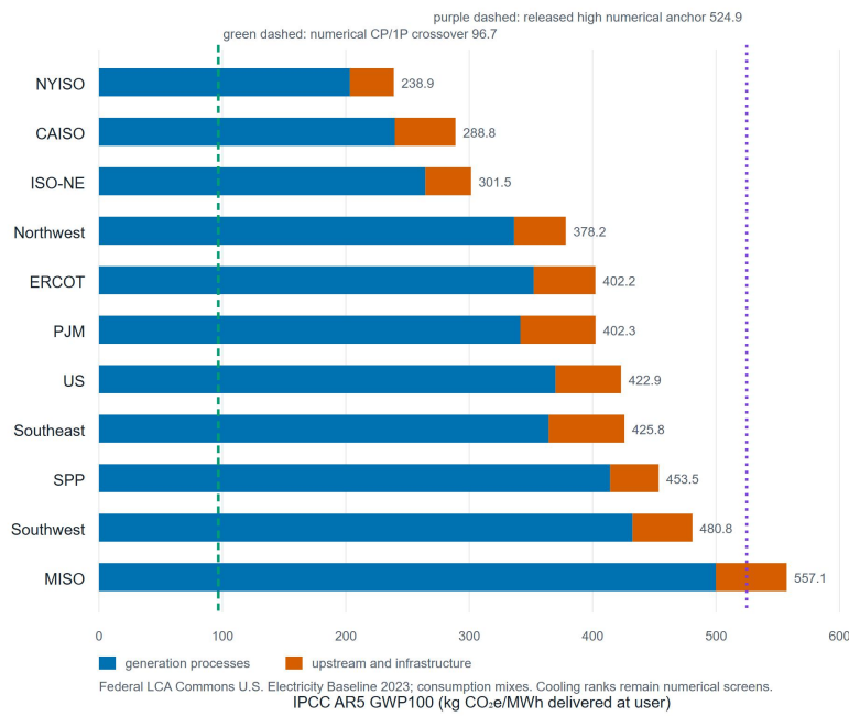
Figure 4: IPCC AR5-GWP100 partial linked-system electricity factors for 10 FERC regions and the United States. The horizontal axis is kg CO 2 e/MWh delivered at the user. Bars separate generation-process impacts from other linked upstream and infrastructure impacts. The green dashed line marks the 96.704 kg CO 2 e/MWh released-workbook numerical crossover. The purple dashed line marks the 524.893 kg CO 2 e/MWh released high numerical anchor. Neither line creates method equivalence or a facility decision threshold.
