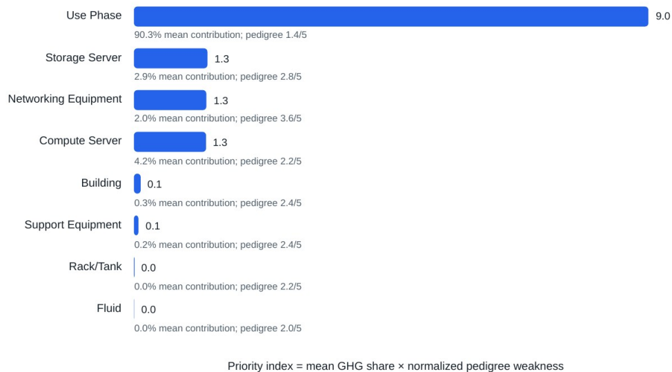
Figure 4. Contribution-weighted evidence-improvement priority derived from the released Microsoft/WSP grid-case GHG contributions and pedigree matrix. The diagnostic multiplies mean contribution share by normalized pedigree weakness; it is a transparent screening rank, not a formal expected value of information.
