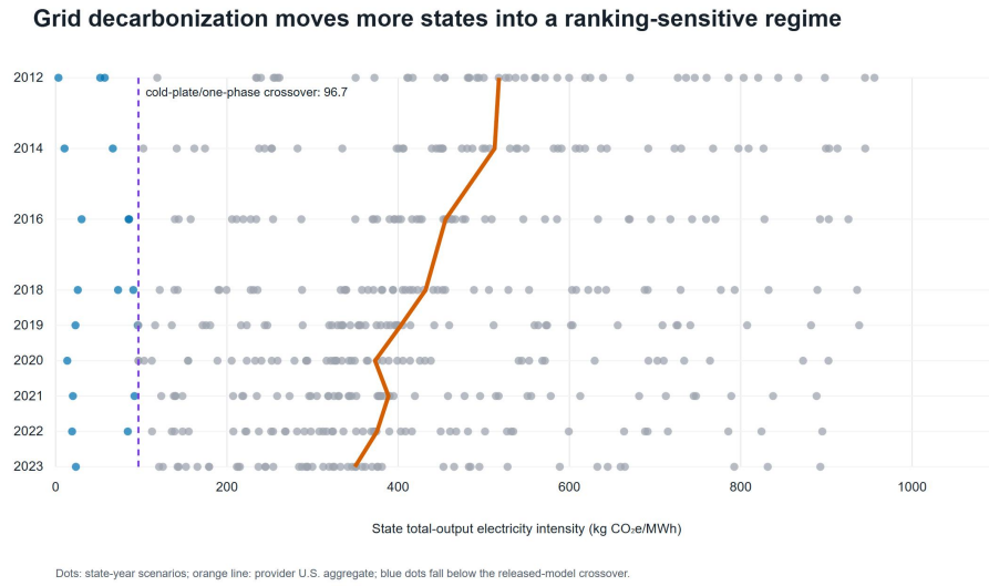
Figure 3: Harmonized AR5-GWP100 eGRID state/DC generation rates for nine releases. Orange denotes the provider U.S. aggregate. Blue points fall below the released-model numerical cold-plate/single-phase crossover. These are direct-generation scenarios, not consumption LCIs or state cooling LCAs.
