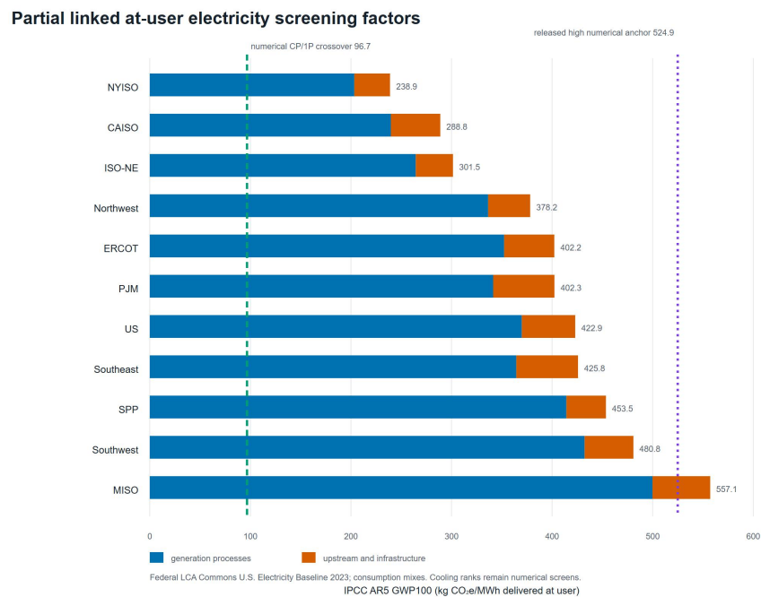
Figure 4: IPCC AR5-GWP100 partial linked-system electricity factors for 10 FERC regions and the United States. Bars separate generation-process impacts from other linked upstream and infrastructure impacts. Vertical lines show the two released numerical cooling landmarks; they do not create method equivalence.
