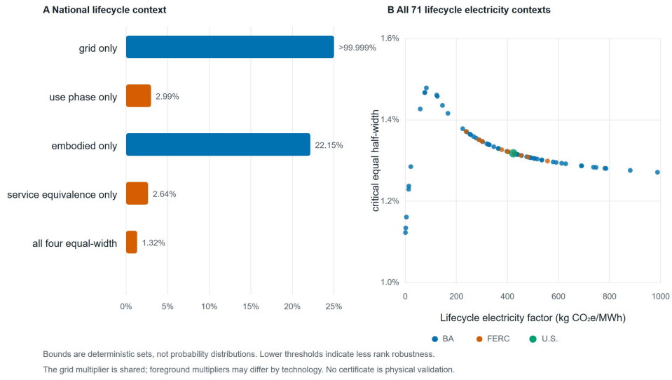
Figure 5: Deterministic equal-width rank-robustness certificates. (A) National critical half-width by active block. (B) all-block thresholds across 60 balancing authorities, 10 FERC regions, and the national system. Bounds are uncertainty sets, not probability distributions or physical validation.
