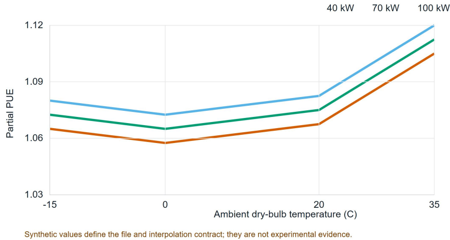
Figure S6: Synthetic load-temperature cooling surface used to verify bounded interpolation. No comparative assertion is permitted from this fixture.
