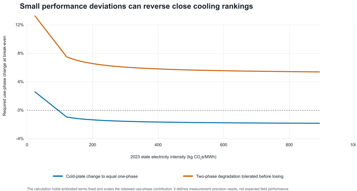
Figure 5. Use-phase break-even stress tests across 2023 state electricity intensities. The blue curve is the cold-plate use-phase change required to equal one-phase immersion; negative values require improvement. The orange curve is the two-phase use-phase increase tolerated before losing first rank. Embodied terms are held fixed. The analysis defines required discrimination and robustness within the released model, not expected field performance.
