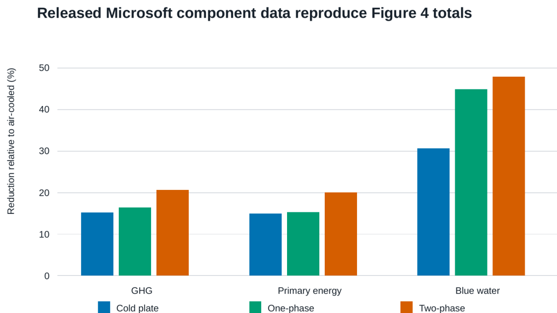
Figure 2. Reconstructed reductions relative to the air-cooled case for the grid scenario in the released Microsoft/Nature source data. Values are derived from published normalized component contributions and validate arithmetic consistency, not proprietary background inventories or foreground bills of materials.
