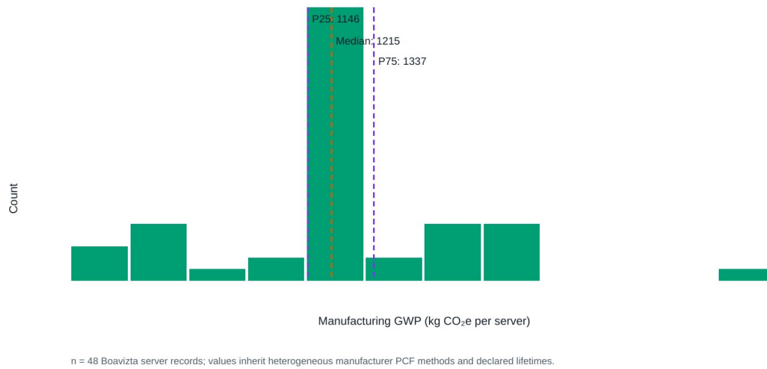
Figure 7. Distribution of manufacturing GHG for 48 Boavizta Datacenter/Server records having total product GHG and manufacturing share. Dashed lines show the 25th percentile, median and 75th percentile. Heterogeneous manufacturer methods and product configurations preclude a product ranking.
