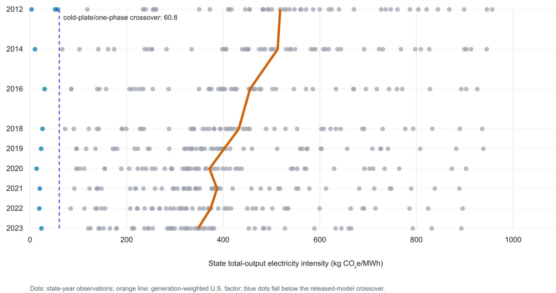
Figure 4. Historical EPA eGRID state total-output intensities for nine releases between 2012 and 2023. Each dot is a state-year observation; the orange line is the generation-weighted U.S. factor. Blue points fall below the 60.8 kg CO 2 e MWh -1 cold-plate/one-phase crossover derived from the released Microsoft/WSP foreground model. The panel describes released annual conditions, not a forecast or marginal-emissions trajectory.
