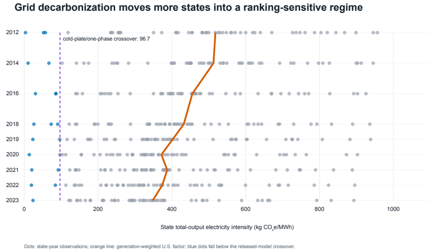
Figure 4: Historical EPA eGRID state total-output intensities for nine releases between 2012 and 2023. Each dot is a state-year electricity-factor scenario; the orange line is the generation-weighted U.S. factor. Blue points fall below the 96.7 kg CO 2 e MWh -1 cold-plate/one-phase crossover derived from the released Microsoft/WSP foreground model. The panel describes released annual generation conditions, not consumption, a forecast, marginal emissions or independent LCAs.
