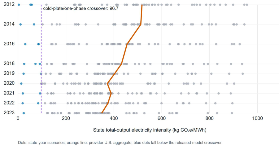
Figure 3: Harmonized AR5-GWP100 eGRID state/DC generation rates for nine releases. Orange denotes the provider U.S. aggregate. Blue points fall below the released-model numerical cold-plate/single-phase crossover. These are direct-generation scenarios, not consumption LCIs or state cooling LCAs.
