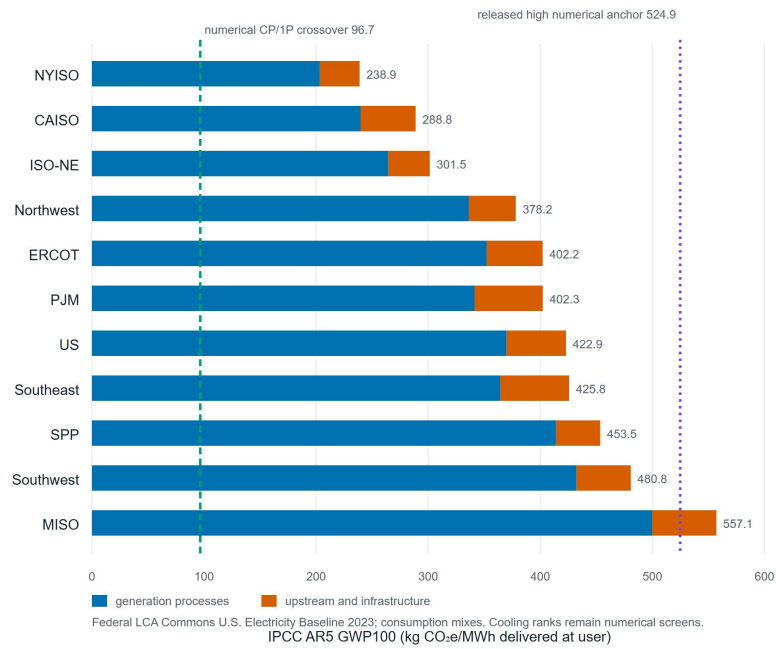
Figure 4: IPCC AR5-GWP100 partial linked-system electricity factors for 10 FERC regions and the United States. Bars separate generation-process impacts from other linked upstream and infrastructure impacts. Vertical lines show the two released numerical cooling landmarks; they do not create method equivalence.
