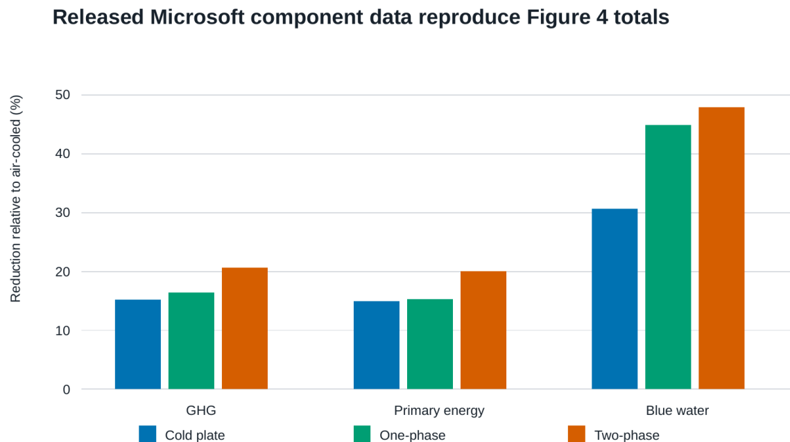
Figure 2. Reconstructed reductions relative to the air-cooled case for the grid scenario in the released Microsoft/Nature source data. Values are derived from published normalized component contributions and validate arithmetic consistency, not proprietary background inventories or foreground bills of materials.
